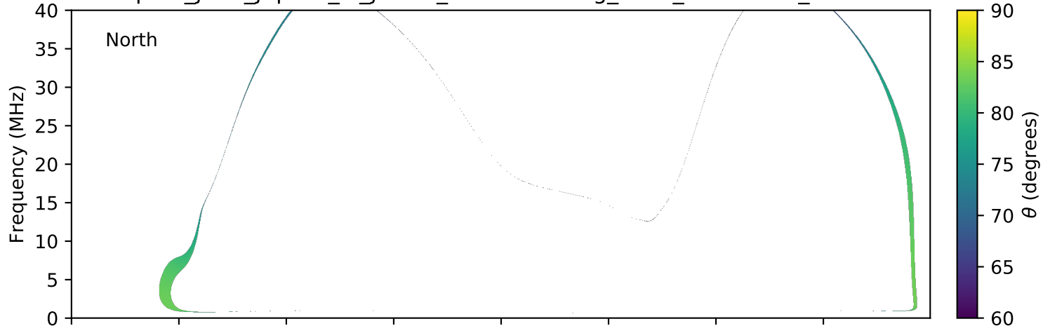
expres_juno_jupiter_io_jrm09_lossc-wid1deg_3kev_20160206_v01.cdf
