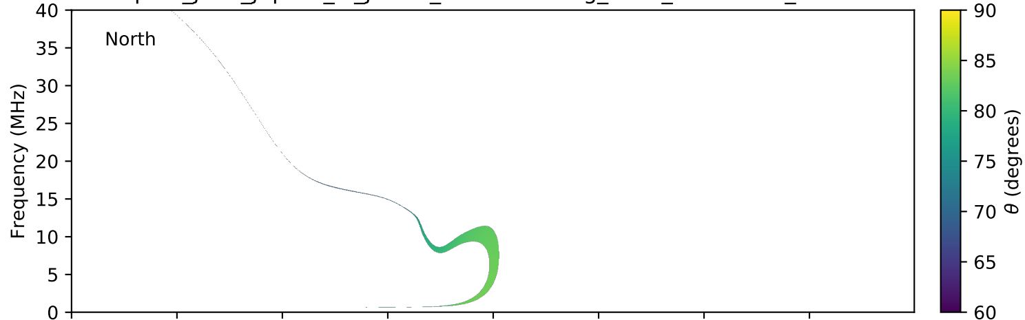
expres_juno_jupiter_io_jrm09_lossc-wid1deg_3kev_20160203_v01.cdf
