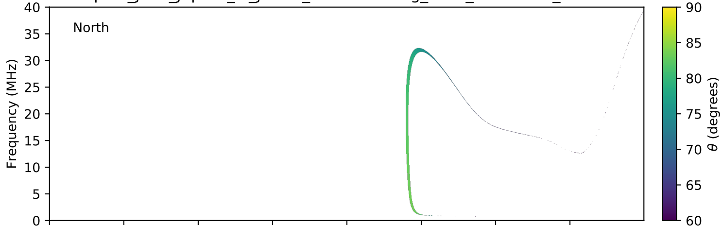
expres_juno_jupiter_io_jrm09_lossc-wid1deg_3kev_20160202_v01.cdf
