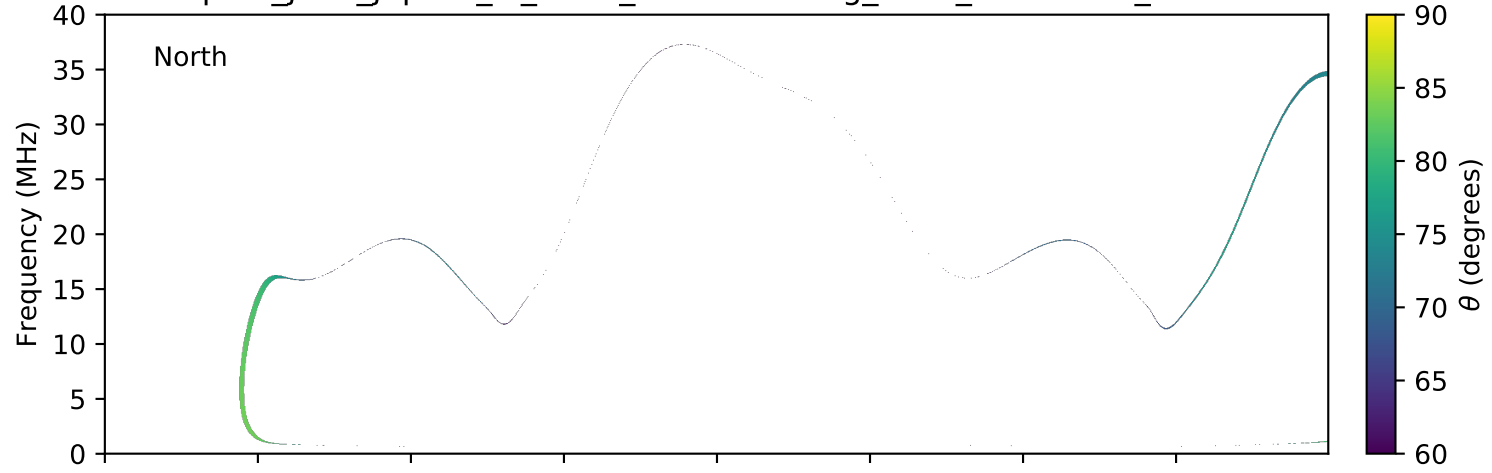
expres_juno_jupiter_io_isaac_lossc-wid1deg_3kev_20160229_v01.cdf
