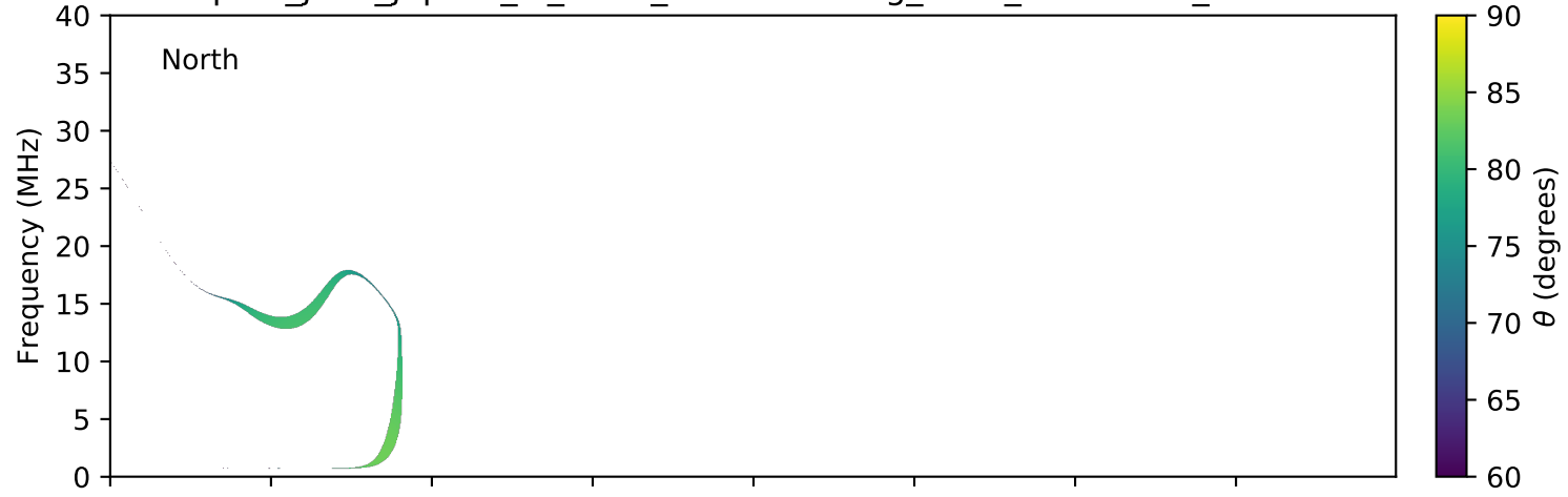
expres_juno_jupiter_io_isaac_lossc-wid1deg_3kev_20160228_v01.cdf
