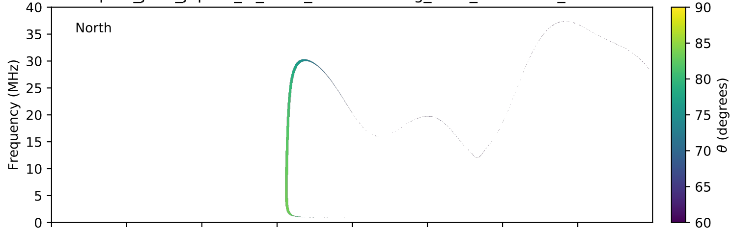
expres_juno_jupiter_io_isaac_lossc-wid1deg_3kev_20160227_v01.cdf
