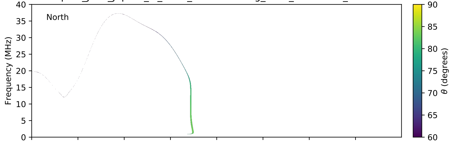
expres_juno_jupiter_io_isaac_lossc-wid1deg_3kev_20160226_v01.cdf
