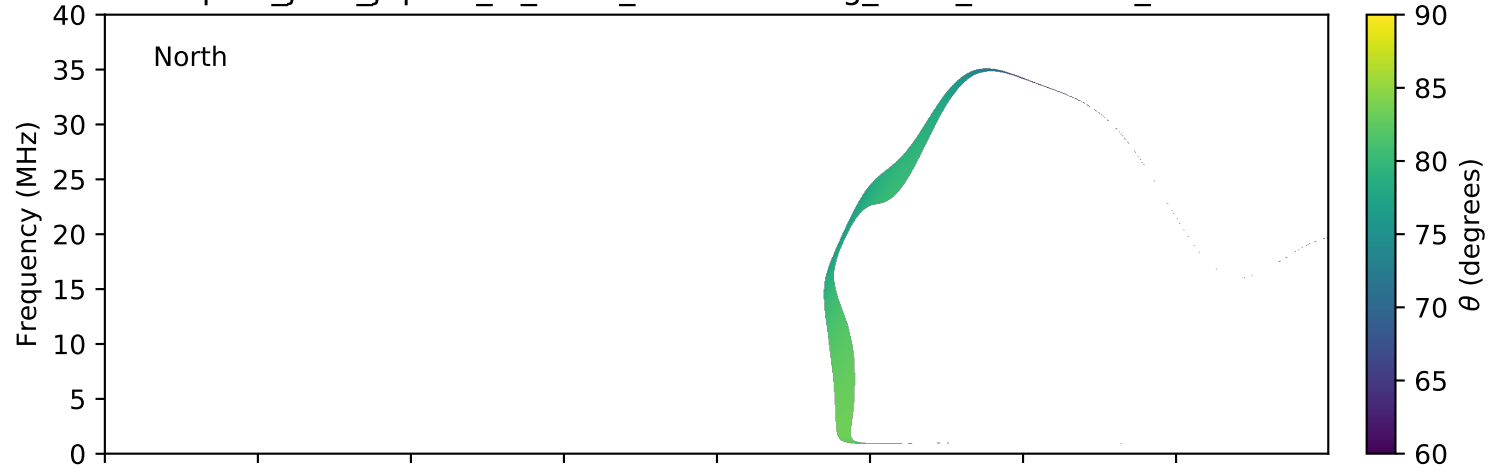
expres_juno_jupiter_io_isaac_lossc-wid1deg_3kev_20160225_v01.cdf
