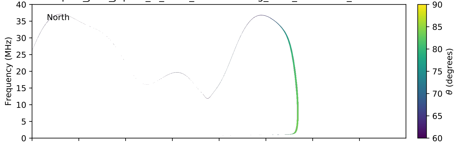
expres_juno_jupiter_io_isaac_lossc-wid1deg_3kev_20160224_v01.cdf
