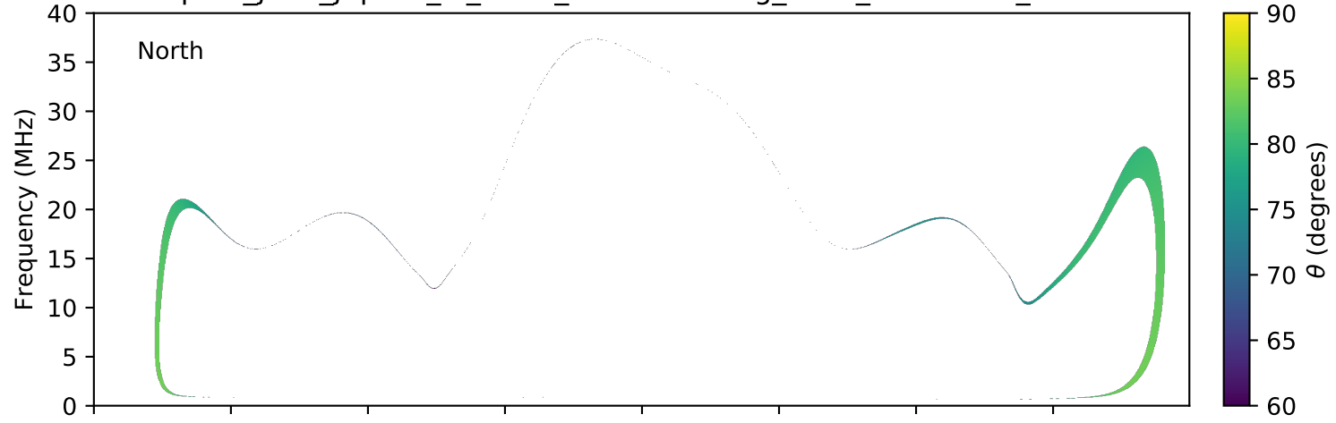
expres_juno_jupiter_io_isaac_lossc-wid1deg_3kev_20160222_v01.cdf
