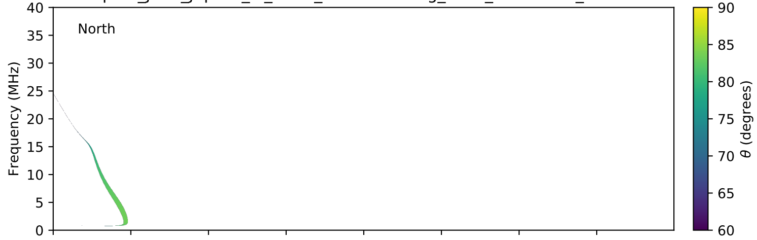
expres_juno_jupiter_io_isaac_lossc-wid1deg_3kev_20160221_v01.cdf
