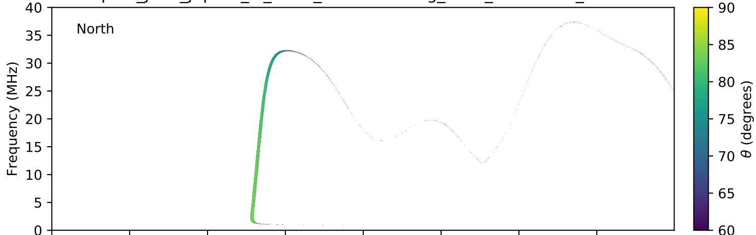
expres_juno_jupiter_io_isaac_lossc-wid1deg_3kev_20160220_v01.cdf
