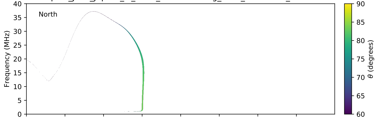
expres_juno_jupiter_io_isaac_lossc-wid1deg_3kev_20160219_v01.cdf
