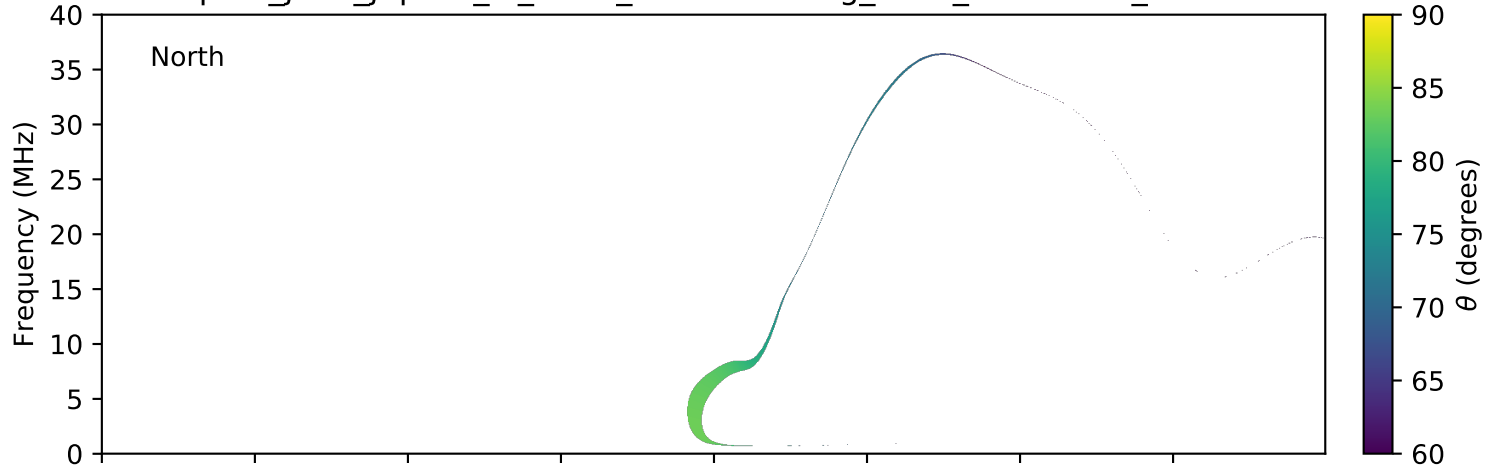
expres_juno_jupiter_io_isaac_lossc-wid1deg_3kev_20160218_v01.cdf
