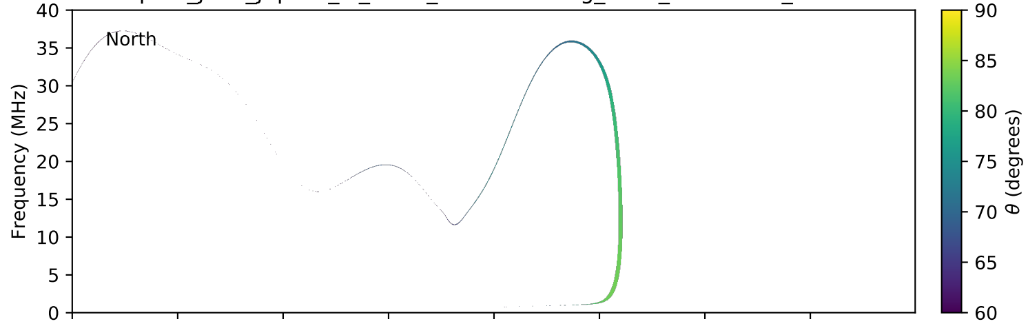
expres_juno_jupiter_io_isaac_lossc-wid1deg_3kev_20160217_v01.cdf
