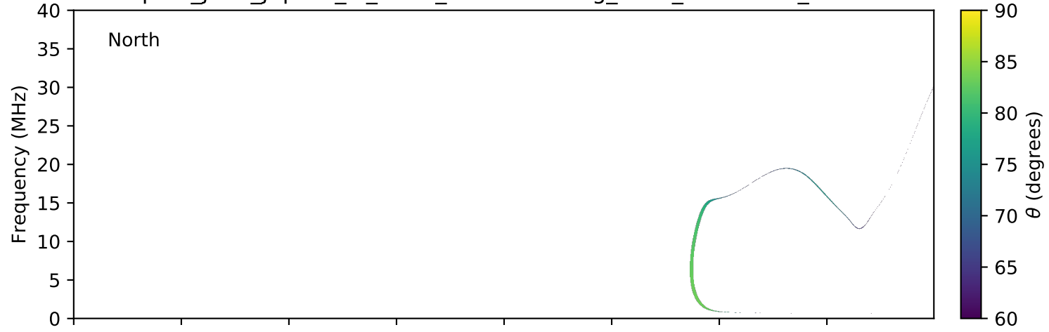
expres_juno_jupiter_io_isaac_lossc-wid1deg_3kev_20160216_v01.cdf
