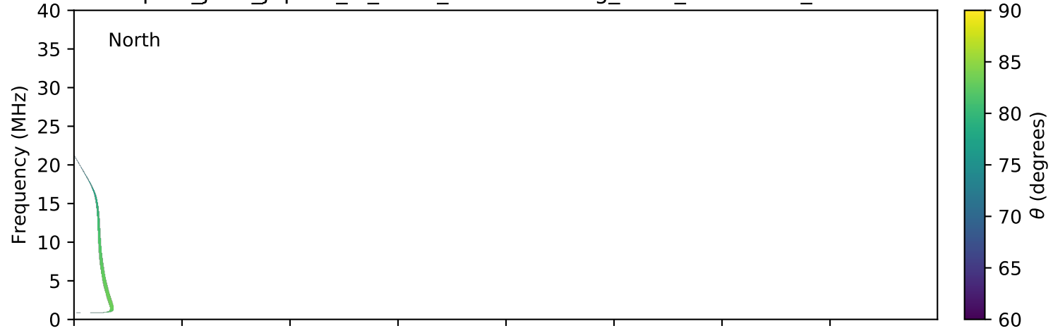
expres_juno_jupiter_io_isaac_lossc-wid1deg_3kev_20160214_v01.cdf
