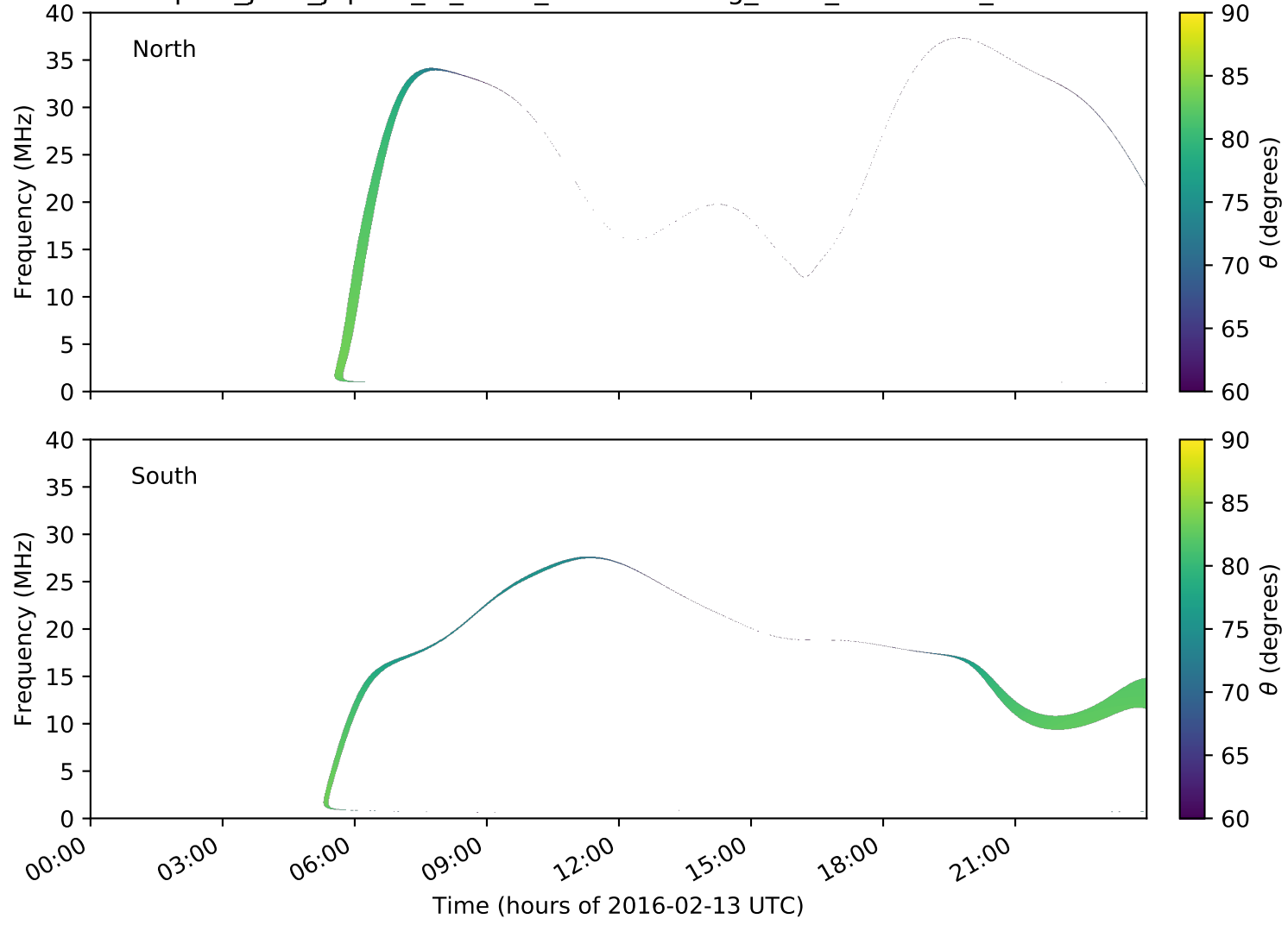
expres_juno_jupiter_io_isaac_lossc-wid1deg_3kev_20160213_v01.cdf
