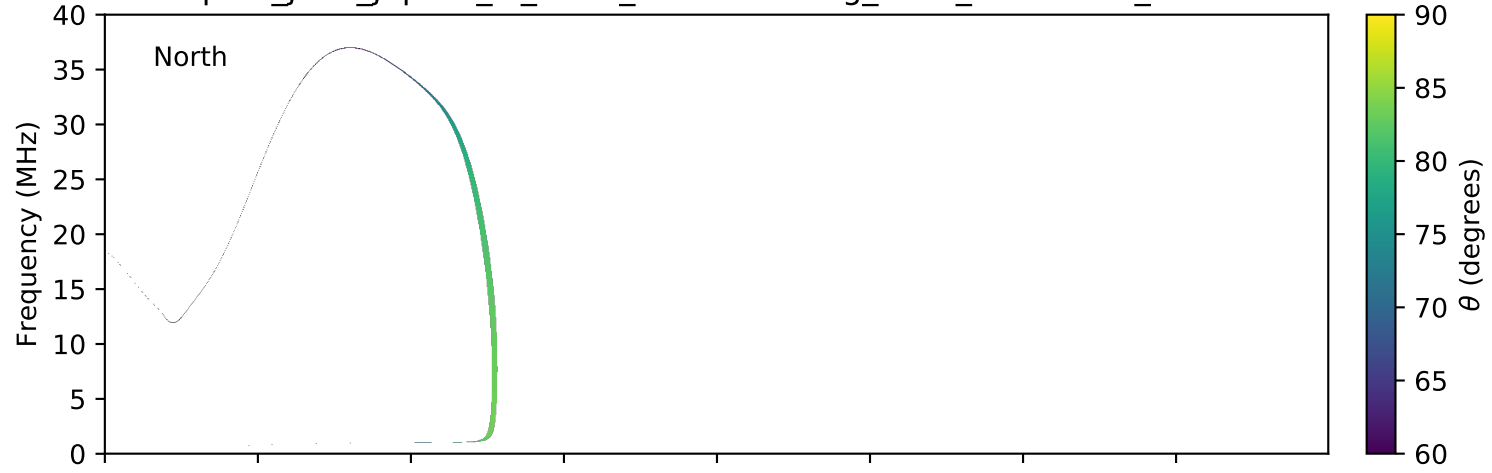
expres_juno_jupiter_io_isaac_lossc-wid1deg_3kev_20160212_v01.cdf
