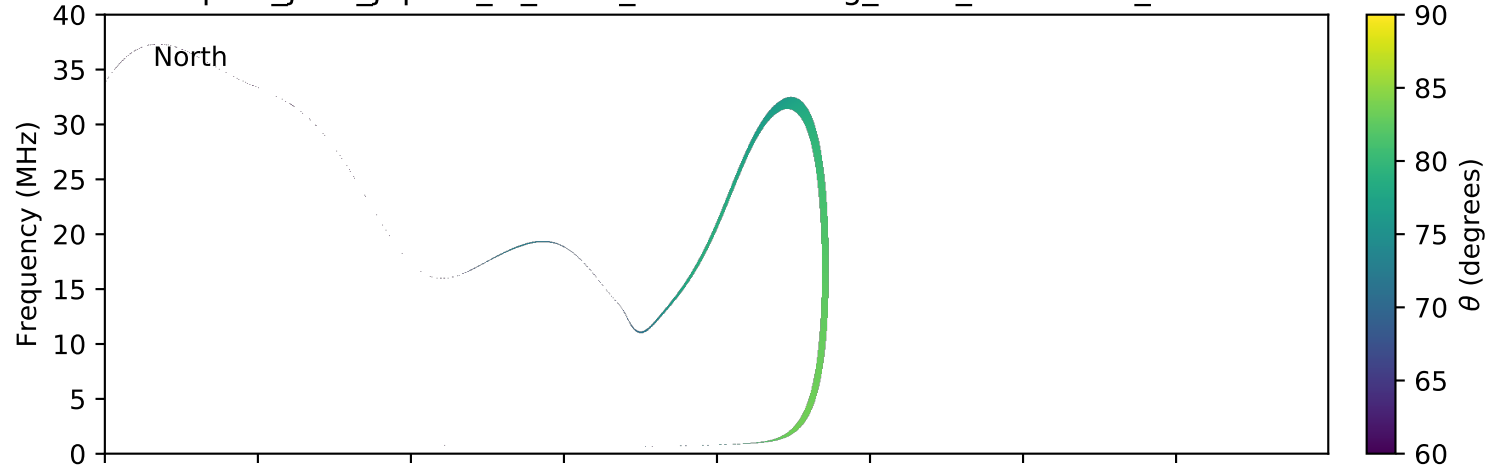
expres_juno_jupiter_io_isaac_lossc-wid1deg_3kev_20160210_v01.cdf
