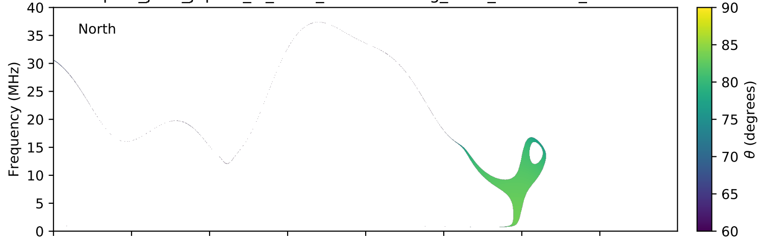
expres_juno_jupiter_io_isaac_lossc-wid1deg_3kev_20160208_v01.cdf
