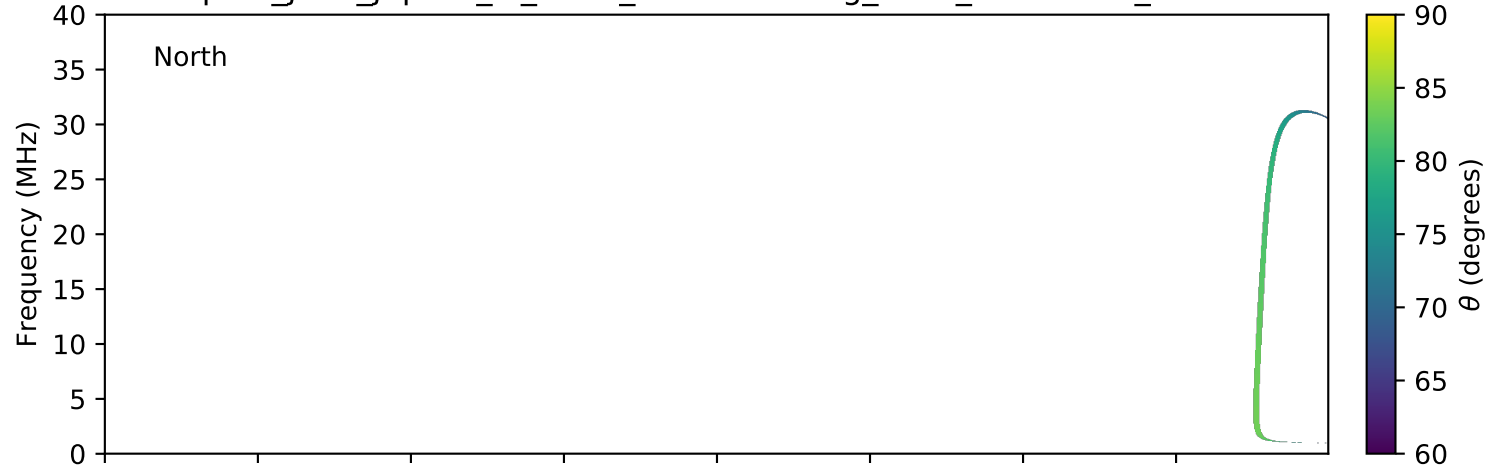
expres_juno_jupiter_io_isaac_lossc-wid1deg_3kev_20160207_v01.cdf
