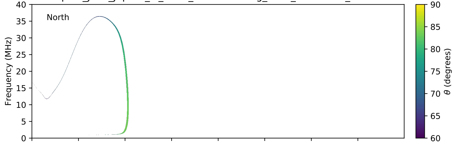
expres_juno_jupiter_io_isaac_lossc-wid1deg_3kev_20160205_v01.cdf
