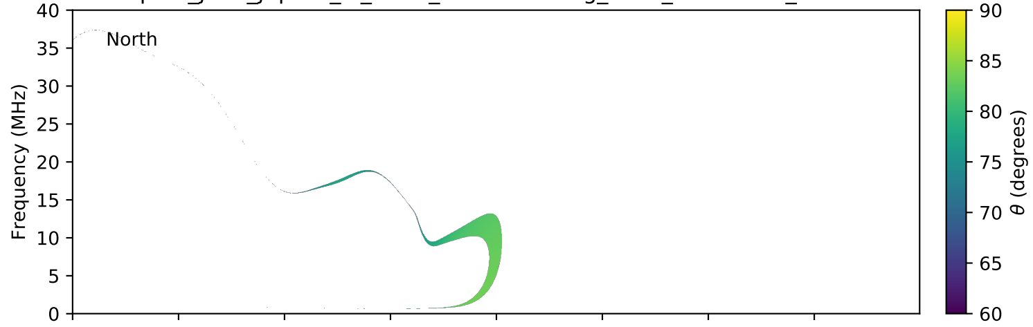
expres_juno_jupiter_io_isaac_lossc-wid1deg_3kev_20160203_v01.cdf
