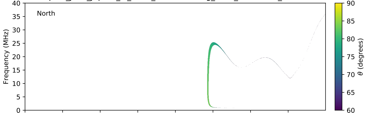
expres_juno_jupiter_io_isaac_lossc-wid1deg_3kev_20160202_v01.cdf
