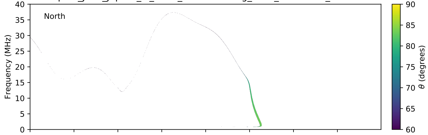
expres_juno_jupiter_io_isaac_lossc-wid1deg_3kev_20160201_v01.cdf
