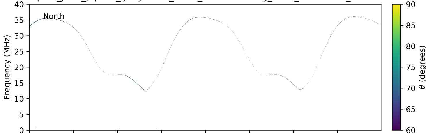
expres_juno_jupiter_ganymede_isaac_lossc-wid1deg_3kev_20160229_v01.cdf
