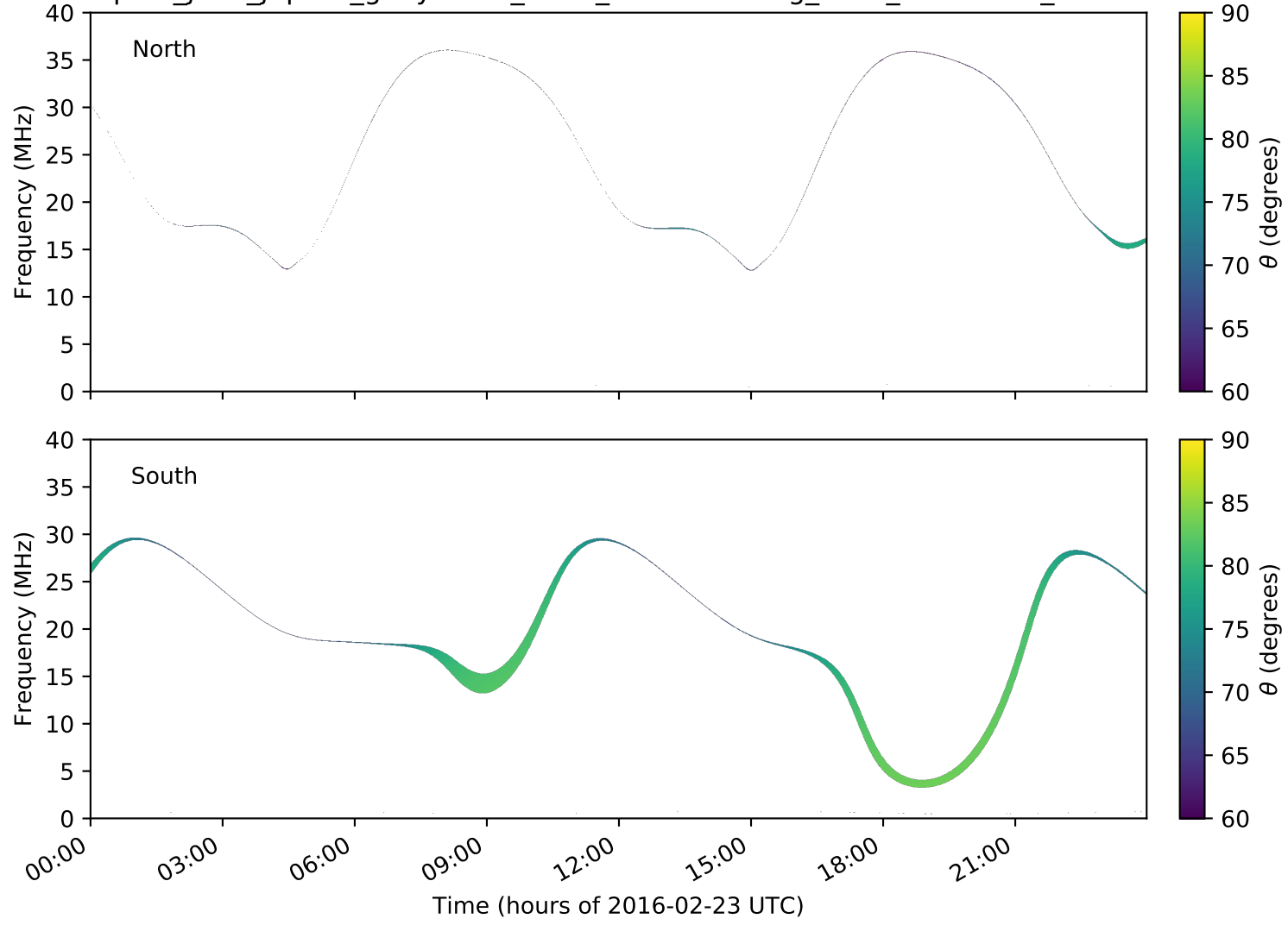
expres_juno_jupiter_ganymede_isaac_lossc-wid1deg_3kev_20160223_v01.cdf
