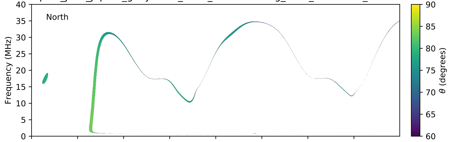
expres_juno_jupiter_ganymede_isaac_lossc-wid1deg_3kev_20160221_v01.cdf
