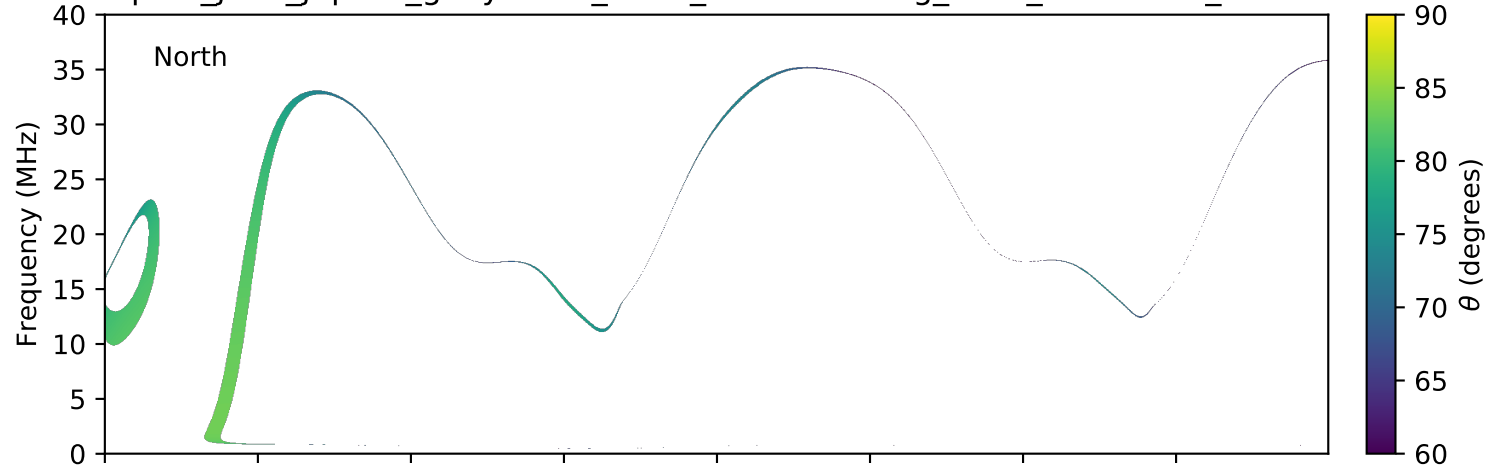
expres_juno_jupiter_ganymede_isaac_lossc-wid1deg_3kev_20160214_v01.cdf
