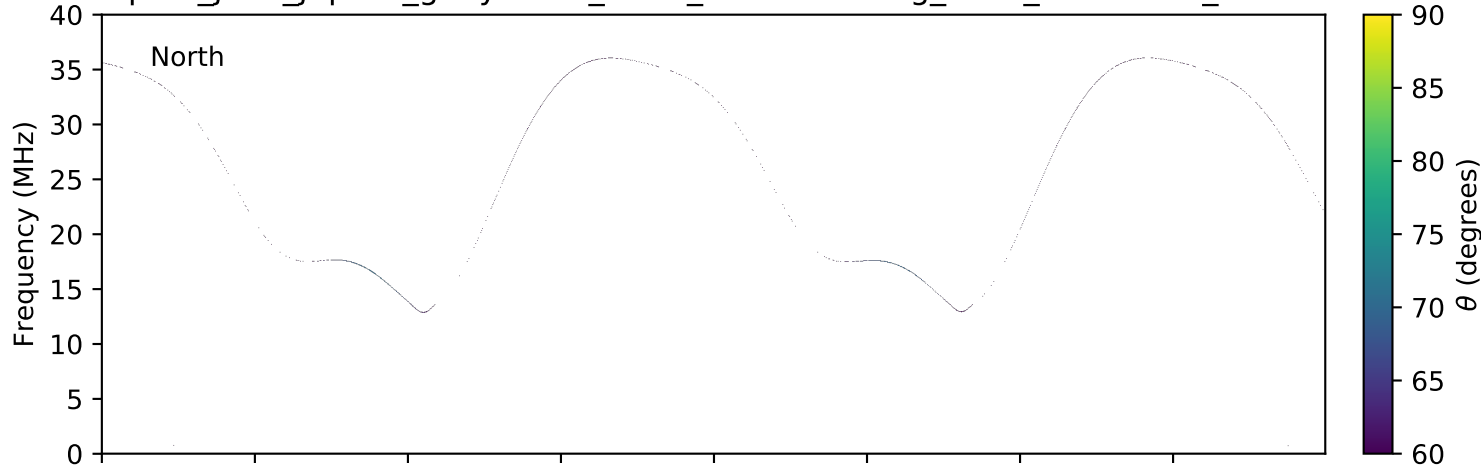
expres_juno_jupiter_ganymede_isaac_lossc-wid1deg_3kev_20160208_v01.cdf
