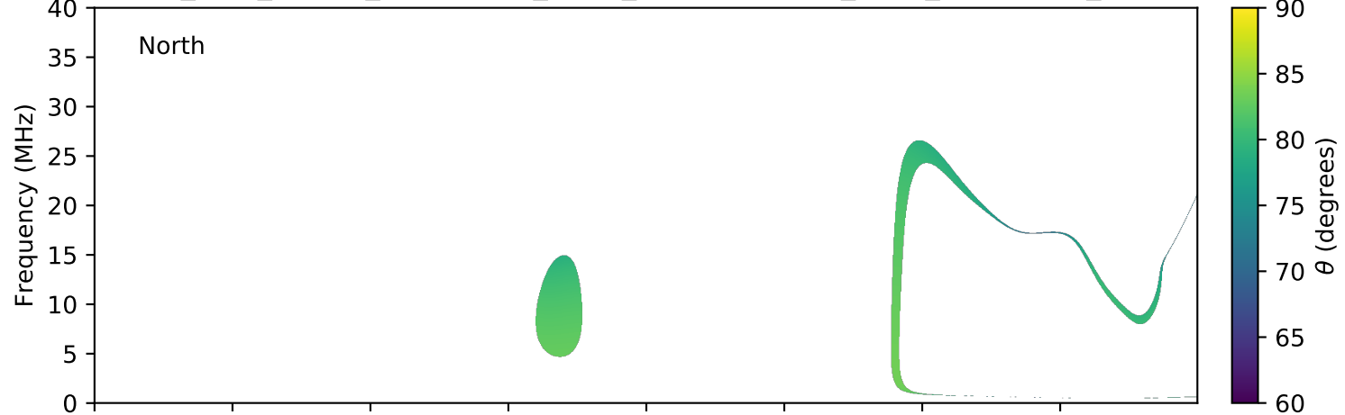
expres_juno_jupiter_ganymede_isaac_lossc-wid1deg_3kev_20160206_v01.cdf
