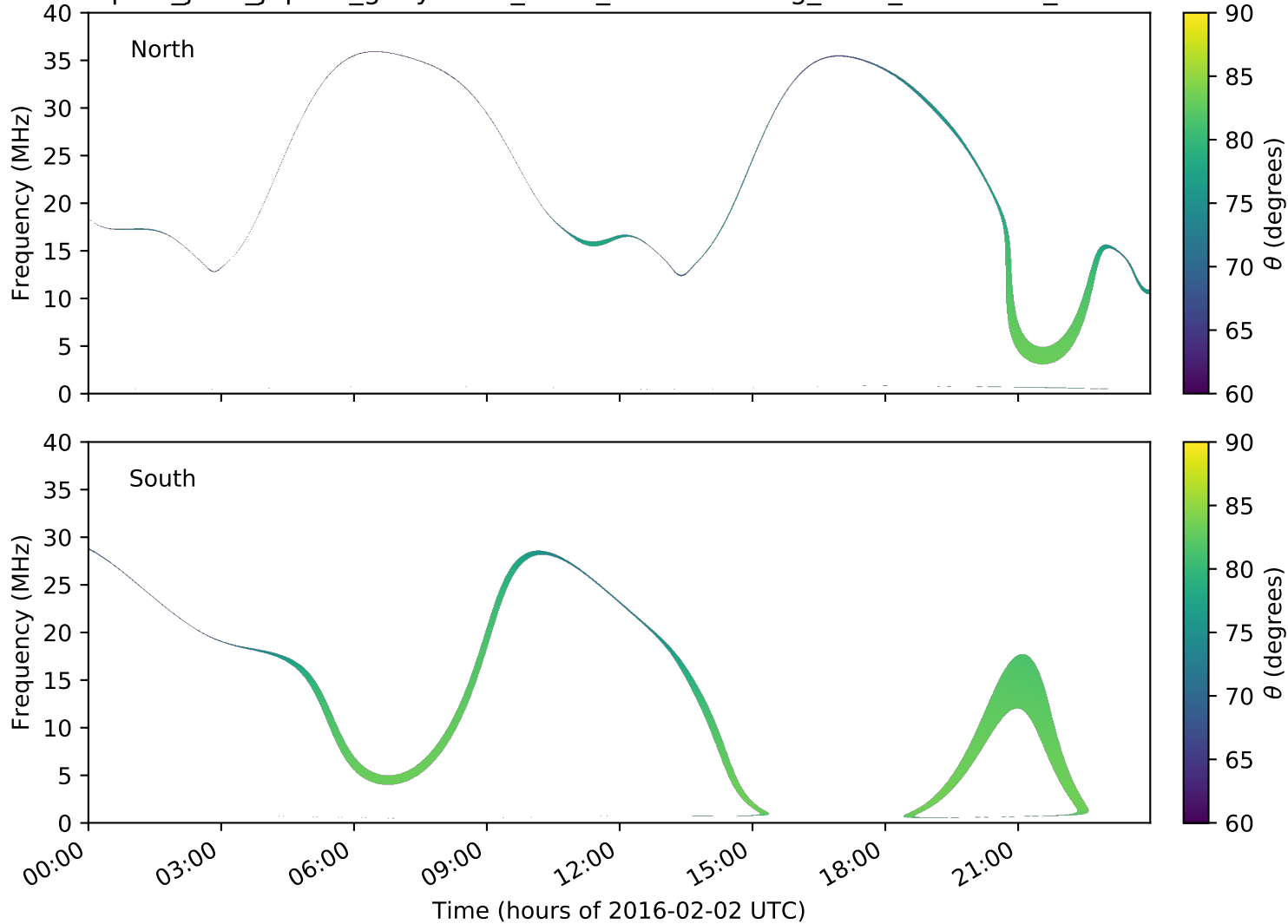
expres_juno_jupiter_ganymede_isaac_lossc-wid1deg_3kev_20160202_v01.cdf
