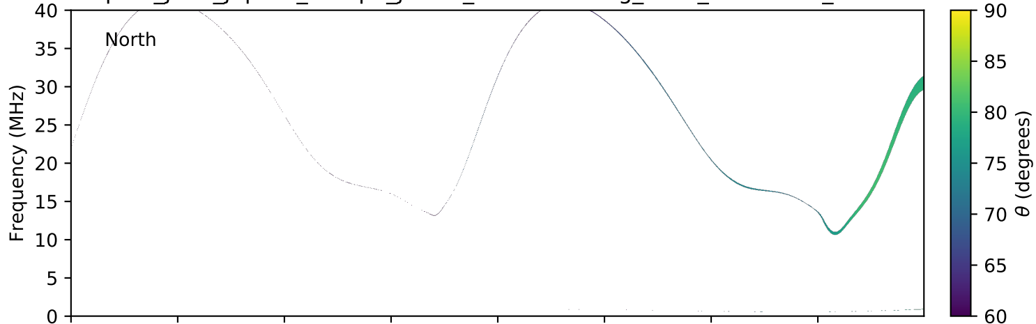
expres_juno_jupiter_europa_jrm09_lossc-wid1deg_3kev_20160229_v01.cdf
