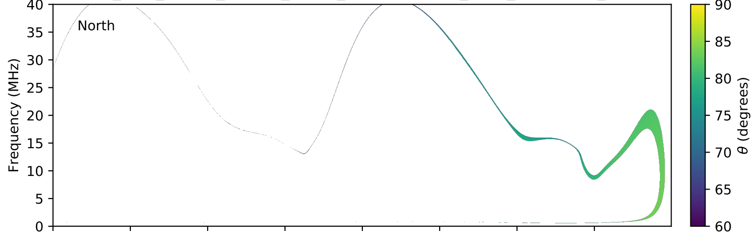
expres_juno_jupiter_europa_jrm09_lossc-wid1deg_3kev_20160222_v01.cdf
