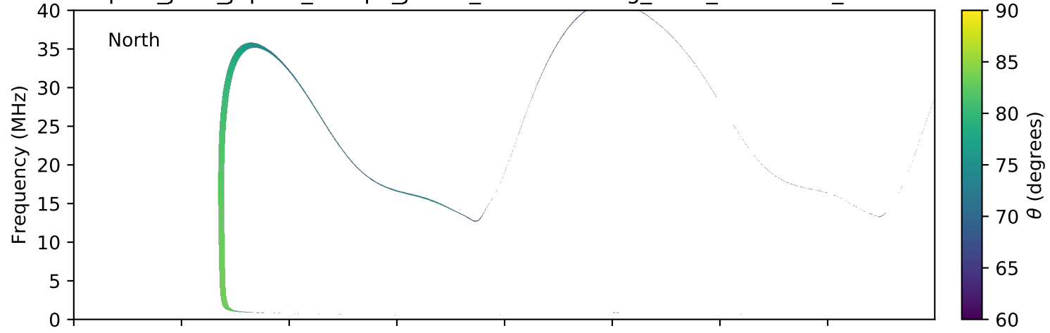
expres_juno_jupiter_europa_jrm09_lossc-wid1deg_3kev_20160221_v01.cdf
