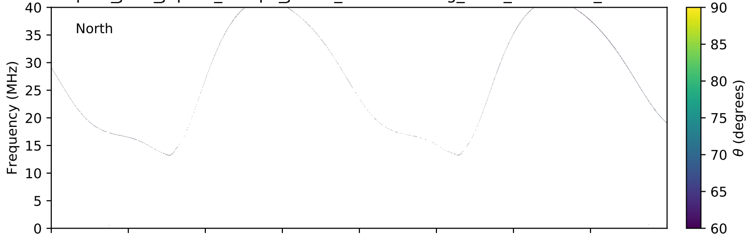
expres_juno_jupiter_europa_jrm09_lossc-wid1deg_3kev_20160218_v01.cdf
