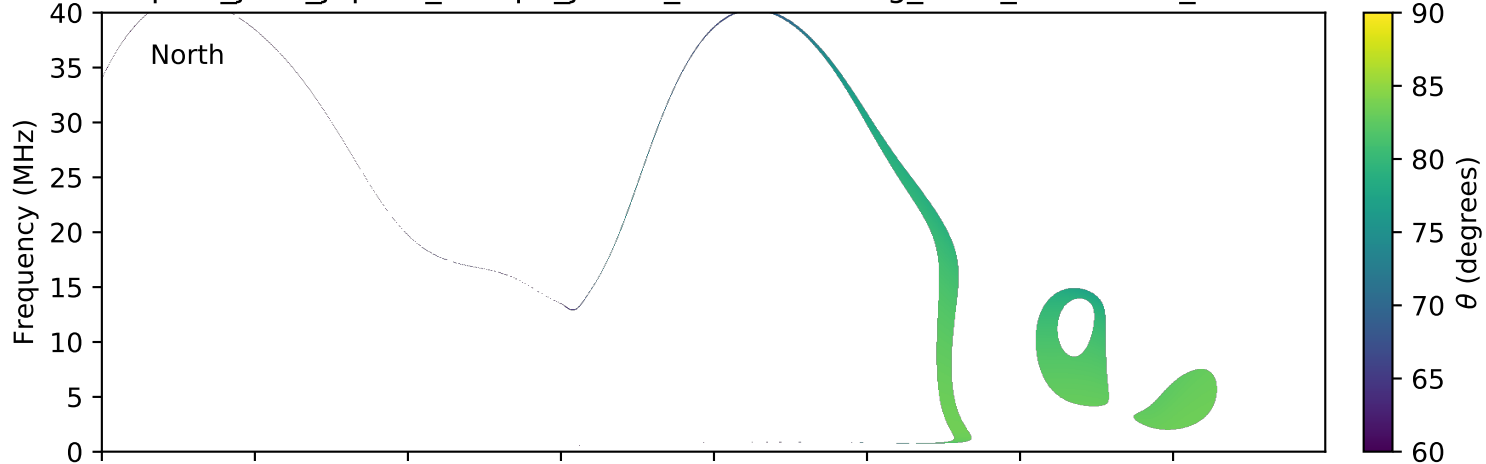
expres_juno_jupiter_europa_jrm09_lossc-wid1deg_3kev_20160215_v01.cdf
