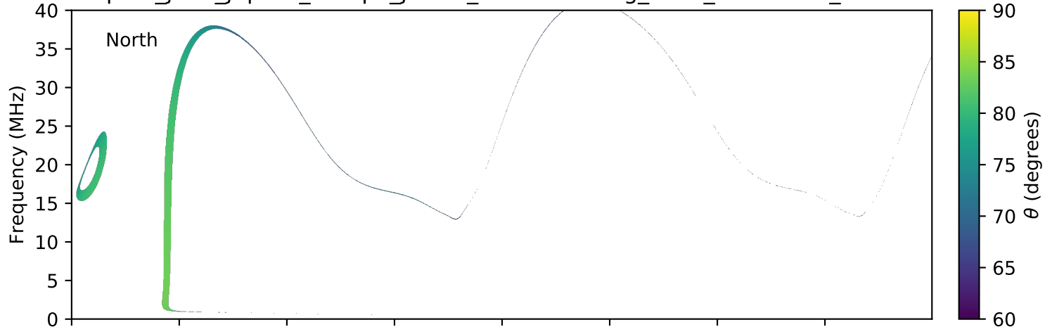
expres_juno_jupiter_europa_jrm09_lossc-wid1deg_3kev_20160214_v01.cdf
