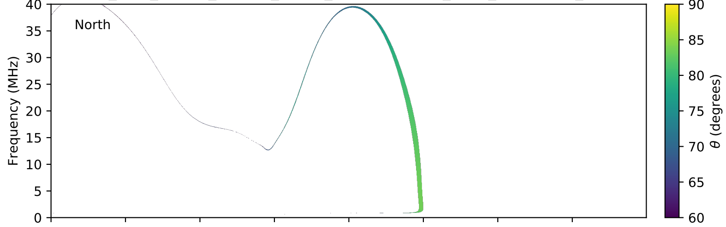
expres_juno_jupiter_europa_jrm09_lossc-wid1deg_3kev_20160208_v01.cdf
