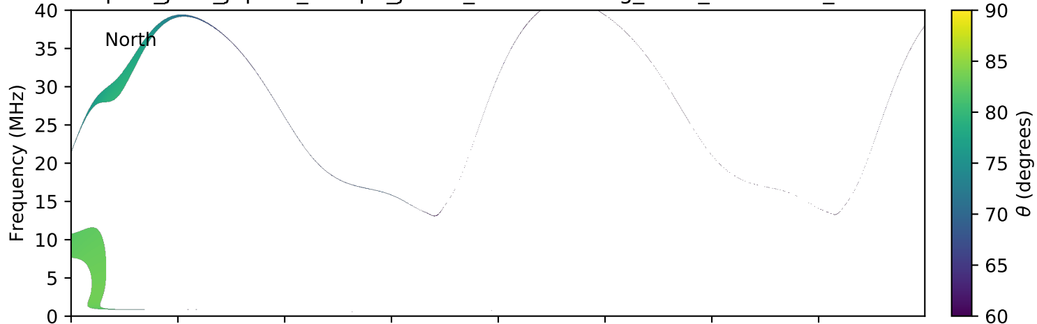
expres_juno_jupiter_europa_jrm09_lossc-wid1deg_3kev_20160207_v01.cdf
