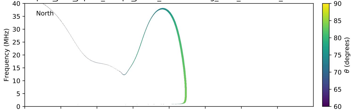
expres_juno_jupiter_europa_jrm09_lossc-wid1deg_3kev_20160201_v01.cdf
