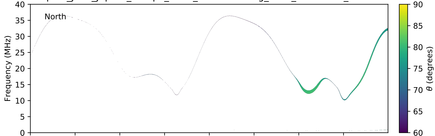
expres_juno_jupiter_europa_isaac_lossc-wid1deg_3kev_20160229_v01.cdf
