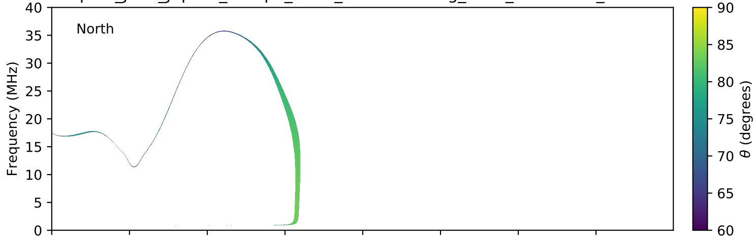
expres_juno_jupiter_europa_isaac_lossc-wid1deg_3kev_20160226_v01.cdf
