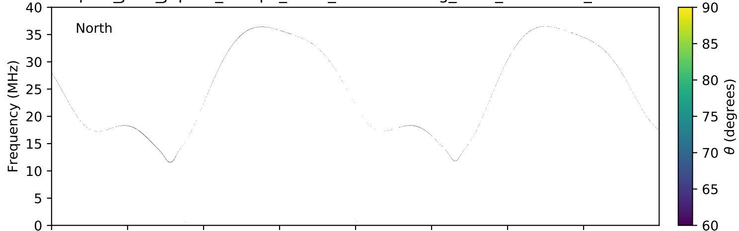
expres_juno_jupiter_europa_isaac_lossc-wid1deg_3kev_20160225_v01.cdf
