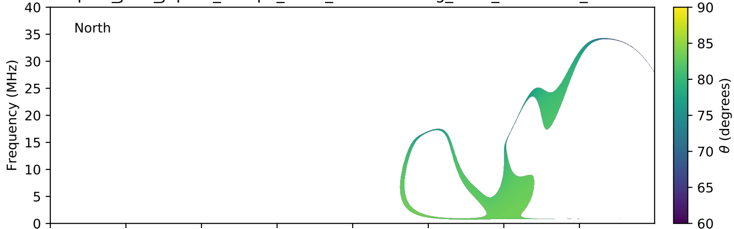
expres_juno_jupiter_europa_isaac_lossc-wid1deg_3kev_20160224_v01.cdf
