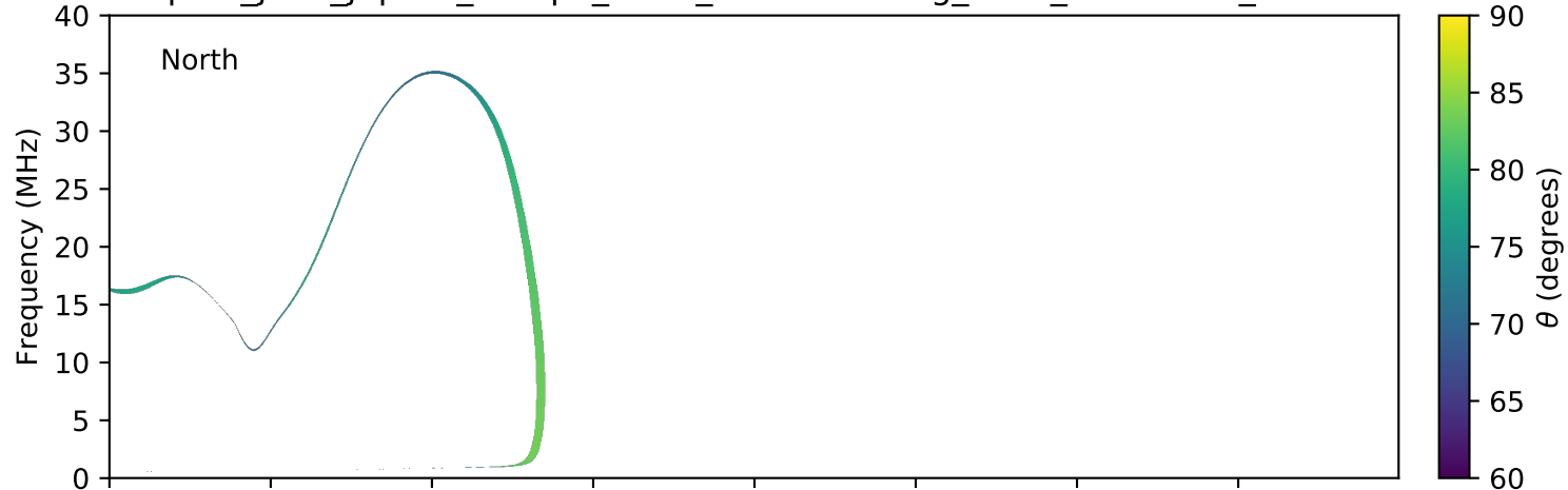
expres_juno_jupiter_europa_isaac_lossc-wid1deg_3kev_20160219_v01.cdf
