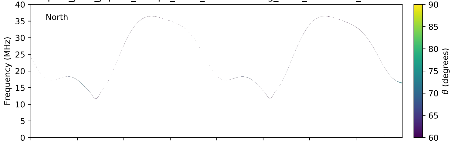
expres_juno_jupiter_europa_isaac_lossc-wid1deg_3kev_20160218_v01.cdf
