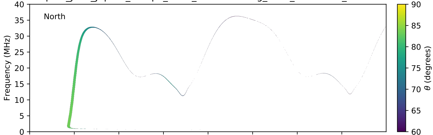
expres_juno_jupiter_europa_isaac_lossc-wid1deg_3kev_20160214_v01.cdf
