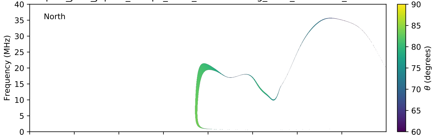
expres_juno_jupiter_europa_isaac_lossc-wid1deg_3kev_20160210_v01.cdf
